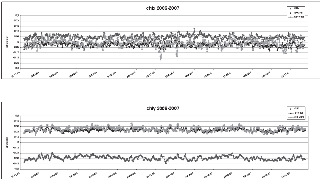
Fig. 3: x-y Excitation Functions 2006 – 2007 from ASI, SBA values
