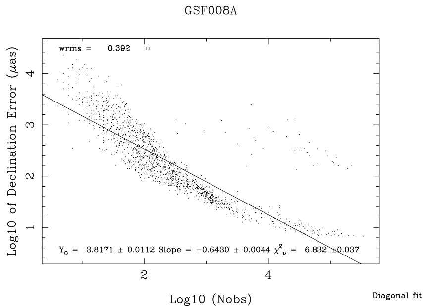
Figure 45: gsf008a catalogue's dependence of un-inflated \sigma_{\delta} on the number of observations for sources observed in at least two sessions. A slope of -0.5 would correspond to 1/\sqrt{N_{obs}} averaging of white noise. Calibrator survey's \approx 2000 single-session densifying sources are not shown.
