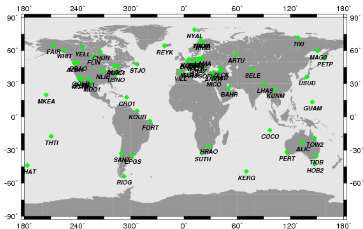
Fig. 5: Network of participating GPS stations in the GRGS project
