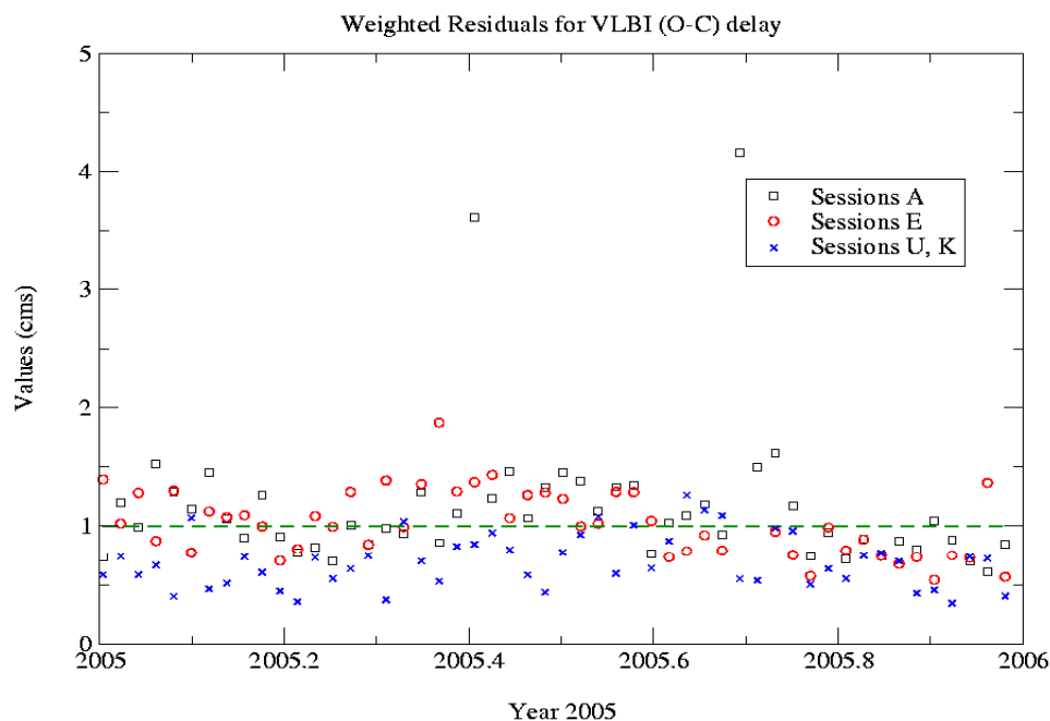
Fig. 7: Weighted residuals for A,E, U and K sessions
