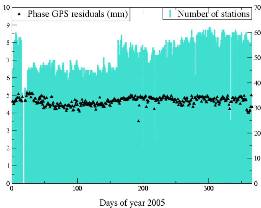
Fig. 6: Number of stations involved in the GPS solution and phase residual in mm
