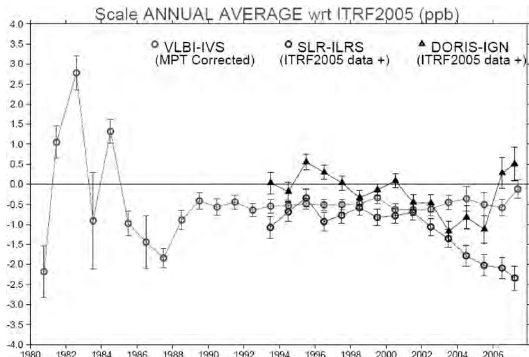
Fig. 1: IVS (mean pole tide correction applied), ILRS (ITRF2005 augmented by recent data) and DORIS-IGN (ITRF2005 augmented by recent data) scale annual averaged variations with respect to ITRF2005.
