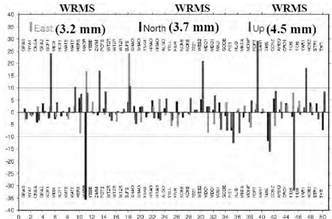
Fig. 2: Local tie residuals as results of an ITRF2005-like combination.
