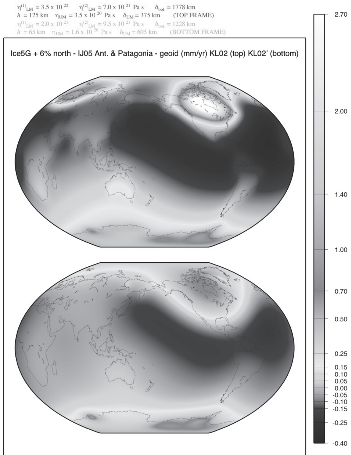
Fig. 1: Variants of the KL02 series, with the lower frame representing a case with the lowest value of upper mantle viscosity represented in the suite of models. It is of interest that Kaufmann and Lambeck (2002) selected the later set (green) parameters when accounting for present-day melting of Antarctica in their modeling scheme.
