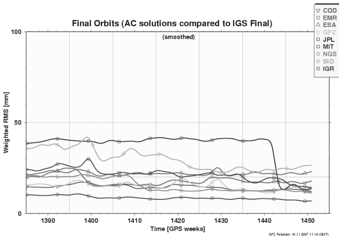
Fig. 2: Weighted RMS differences of all AC's and IGS final orbits to the IGS final combined orbit.
