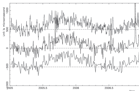
Fig. 7: Plots showing the differences between the GRGS combined solution and combined intra-technique solutions IVS, LRS and IGS for X-pole component over 2005–2006.
