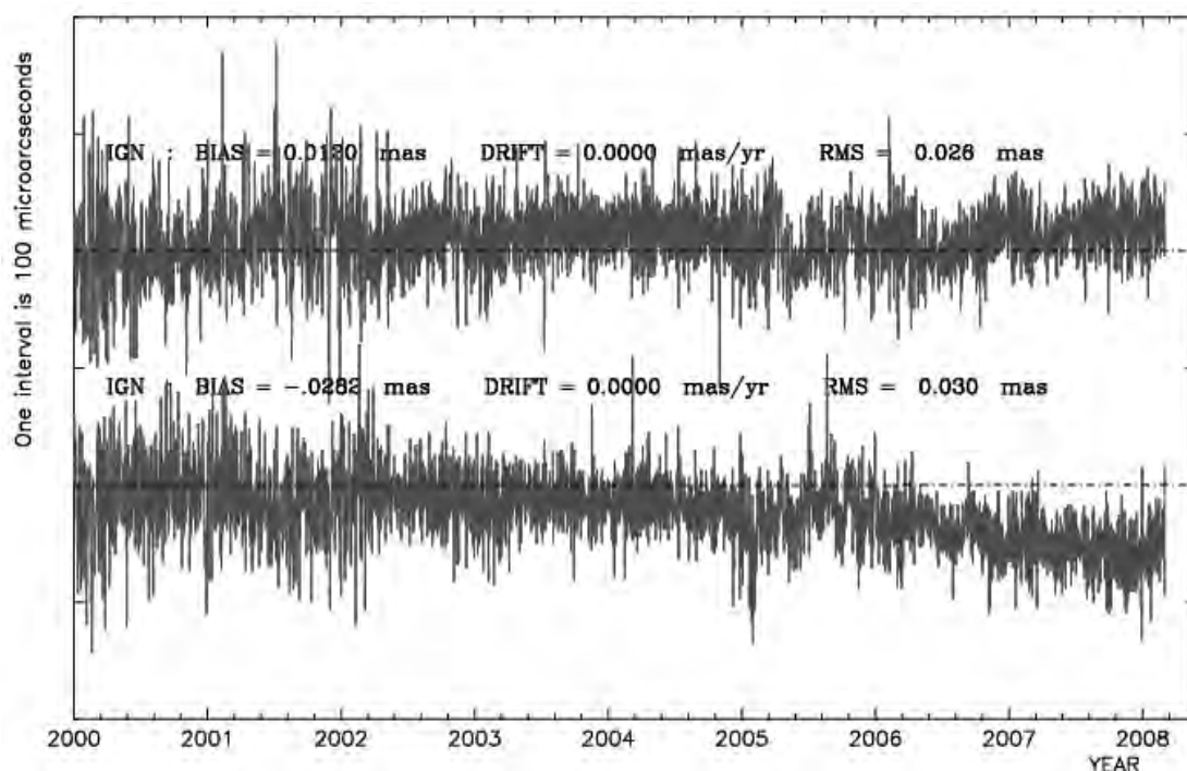
Fig. 1: Polar Motion over 2000–2008, CATREF(2008) – 05 C04
