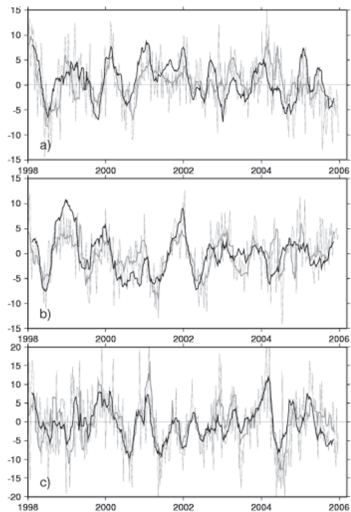
Fig. 1: ILRS solution Helmert parameters from ITRF2005 analysis, in light gray. Estimated parameters constrained with GPS results according to Collilieux et al., 2008, in black. Solid lines correspond to 10 weeks average values. a) X component, b) Y component, c) Z component.
