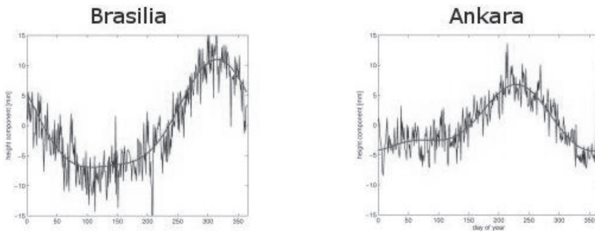
Fig. 4: Shape of the “averaged” annual signal for two ITRF2005 stations. The fitted curve represents the mathematical approximation by annual and semi-annual sine/cosine functions.
