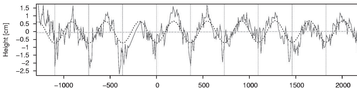
Fig. 3: Seasonal variations for the height component for the GPS station in Irkutsk, Siberia. The time is given in Julian Days (w.r.t. 1.1.2000) from 1996.5 until the end of 2005.
