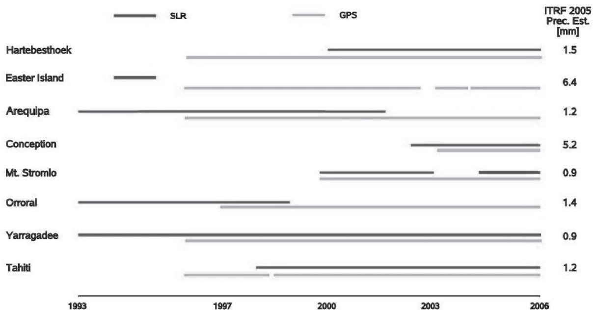
Fig. 2: Observation periods for SLR and GPS co-location sites in the southern hemisphere.
