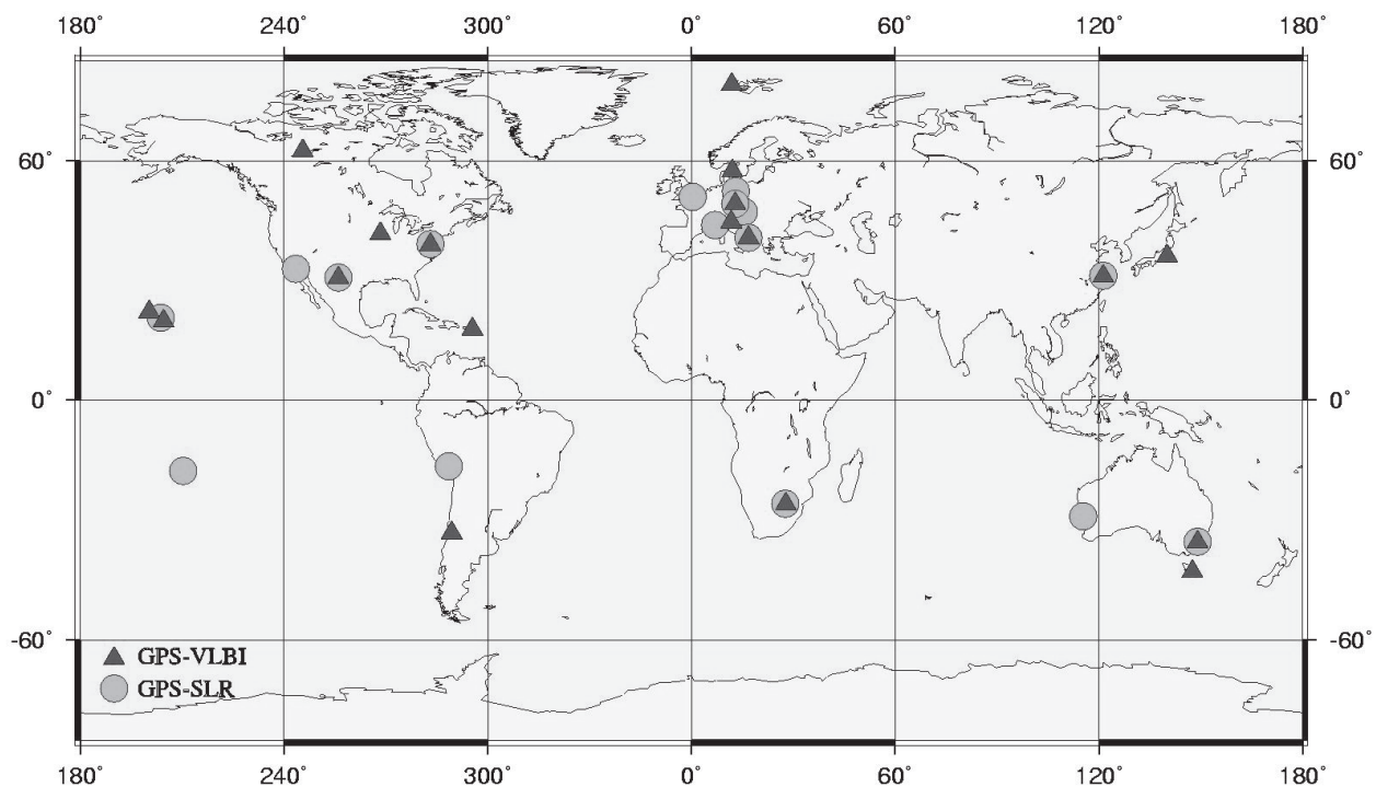
Fig. 1: Distribution of “good” co-location sites between GPS, SLR and VLBI
