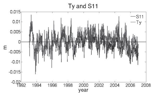
Fig. 4: Y-translation and gravity field coefficient S11.
