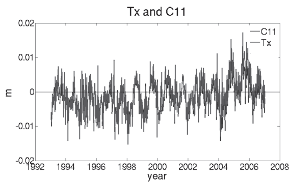
Fig. 3: X-translation and gravity field coefficient C11.
