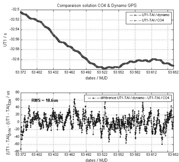
Fig. 3: UT1–TAI 40 cumulated GPS weeks compared to IERS EOP CO4.
