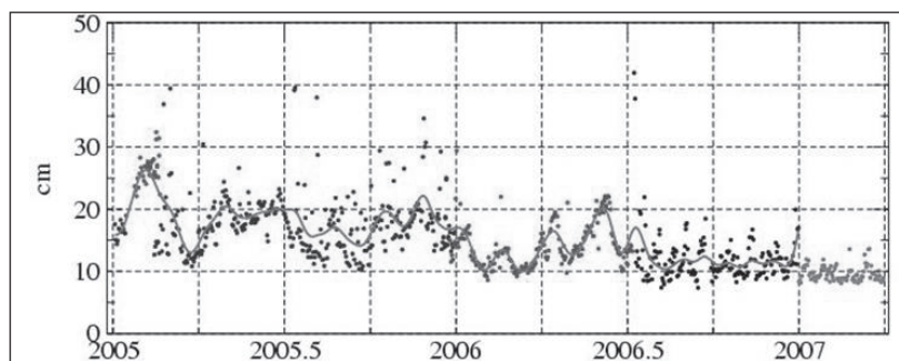
Fig. 1: Internal orbit overlappings (non weighted 3D RMS).
