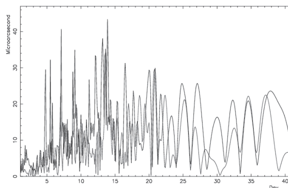
Fig. 9: LSQ periodogram of nutation offsets dx (blue) and dy (red) relatively to MHB2000 nutation model. Significant peaks appear in particular at 7 days and at fortnightly time scales.
