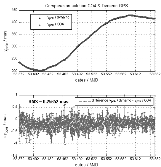
Fig. 2: Y pole 40 cumulated GPS weeks compared to IERS EOP CO4.
