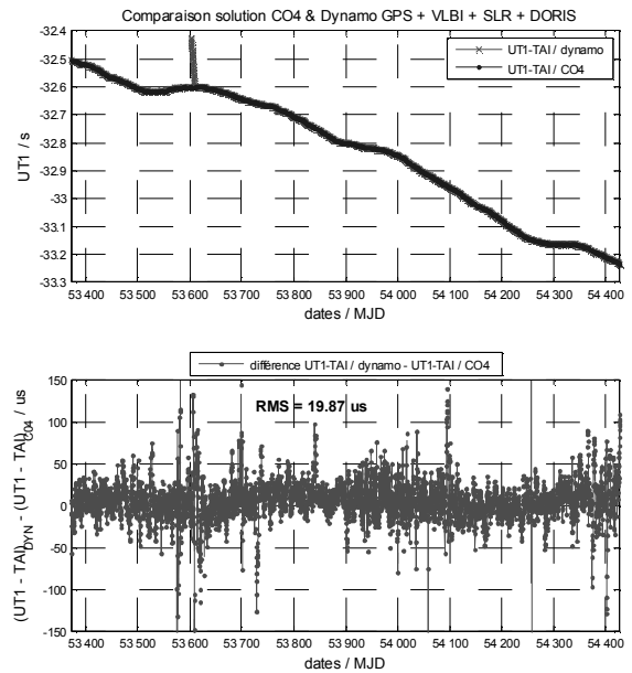
Fig. 5: UT1–TAI compared with IERS EOP CO4, residuals rms = 19.9 \mu s over 2005–2007.
