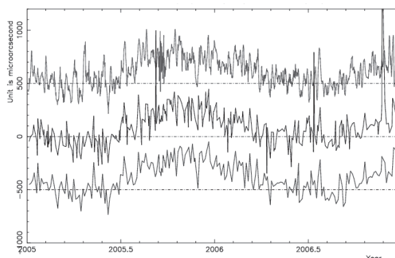
Fig. 7: Plots showing the differences between the GRGS combined solution and combined intra-technique solutions IVS, LRS and IGS for X-pole component over 2005–2006.
