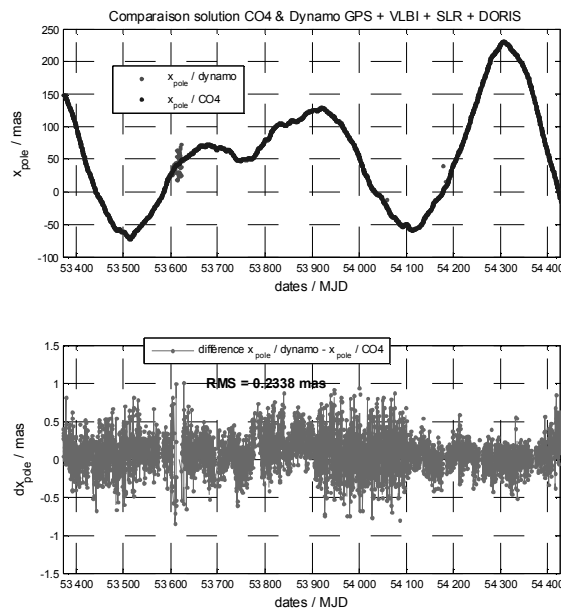
Fig. 4: X pole compared with IERS EOP CO4, residuals rms = 234 \mu s over 2005–2007.
