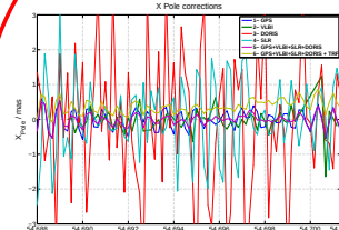
Figure 1 – X-Pole corrections at 6h intervals
