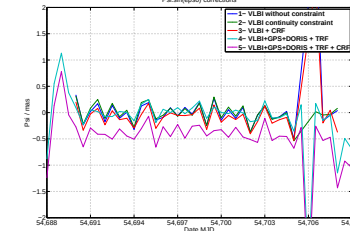
Figure 5: ψ, sin(ε) Nutation longitude corrections at 12h intervals with IAU 1980 model
