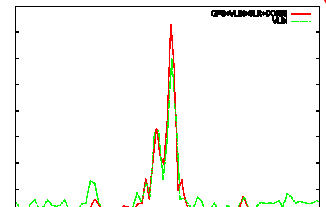
Figure 4 – Pole coordinates spectrum
