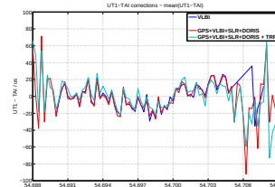
Figure 3 – UT1-TAI corrections at 6h intervals
