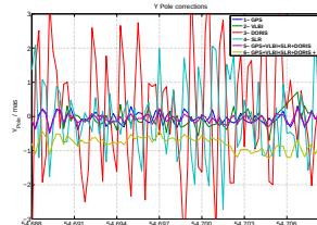
Figure 2 – Y-Pole corrections at 6h intervals
