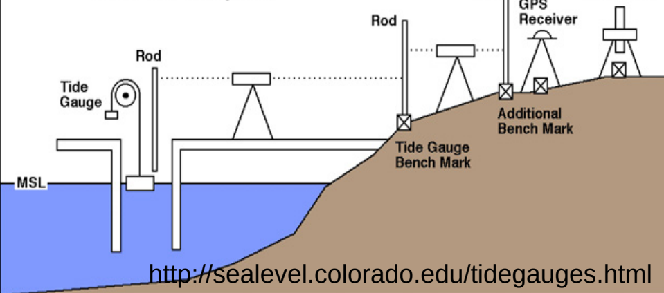
Figure 1: Schematic of a Tide Gauge Measurement System
