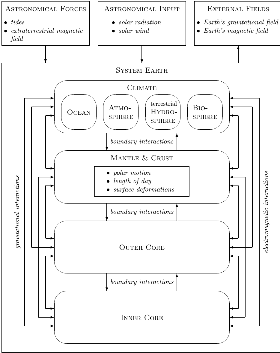
Figure 3. Components of the Earth system and their mechanical interactions. The Earth system can be viewed as composed of subsystems such as crust and mantle, outer and inner cores, and the fluid envelop of the solid Earth. The latter consists of ocean, atmosphere, and terrestrial hydrosphere, which are the prominent components of the climate system. We have chosen not to separate the cryosphere from the ocean and terrestrial hydrosphere but rather consider the ice load on land as part of the terrestrial hydrosphere and sea ice as part of the ocean. The biosphere is also interacting with the components of the climate system, and, considering the anthroposphere as part of the biosphere, also the solid Earth. The subsystems interact through surface forces at the joining boundaries and through volume forces (gravitational and electromagnetic). The overall system is subject to external forces including tidal forces and the extra-terrestrial magnetic field. From Plag (2006a).
