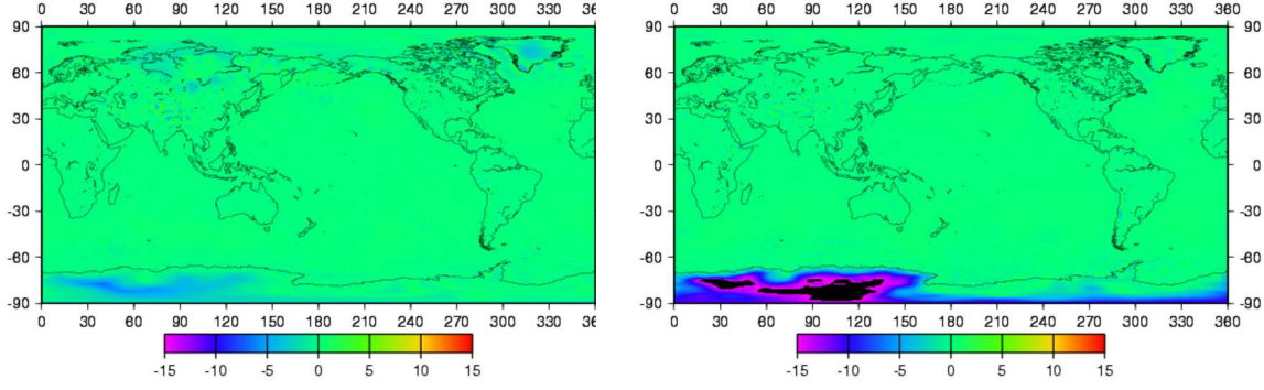
Figure 5. Differences \delta^{\text{geop}} of air pressure at MSL. The quantity shown is \delta^{\text{geop}} as defined by eq. (16). Plots are for 2000/01/01/00 (left) and 2000/08/01/12 (right). Resolution of the datasets is 5 minutes. The scale is in HPa.
