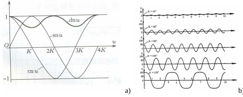
Fig 1. a) Graphs of elliptic functions b) cn u compared with trigonometric \cos u
