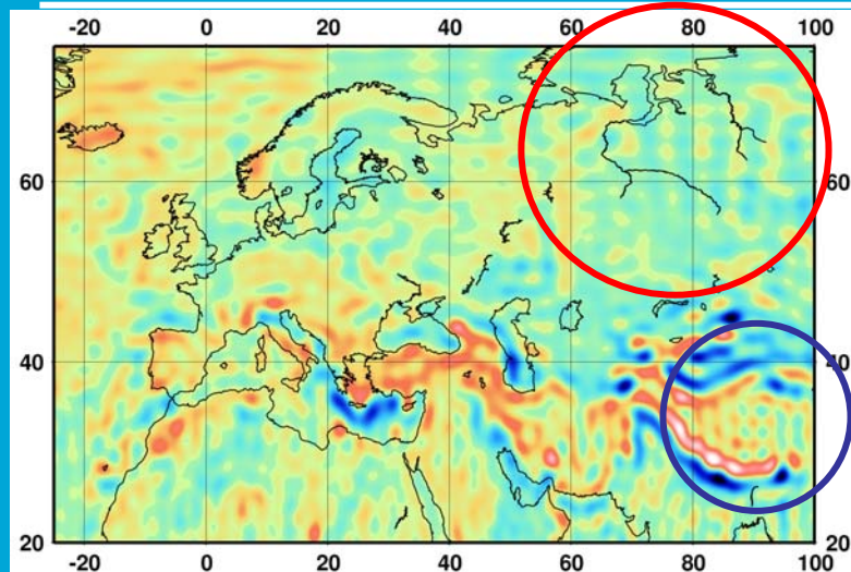
1) GRACE-only until d/o 150 (EIGEN-GL04S1)
