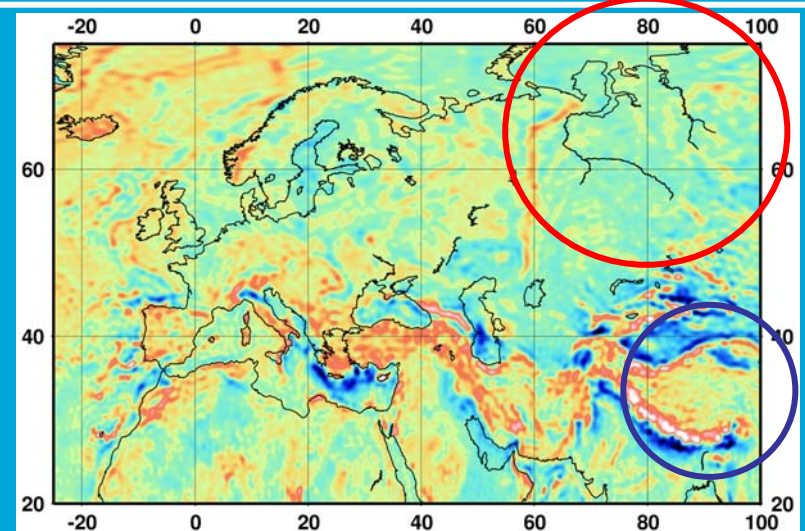
3) GRACE + surface until d/o 360 (EIGEN-GL04C)
