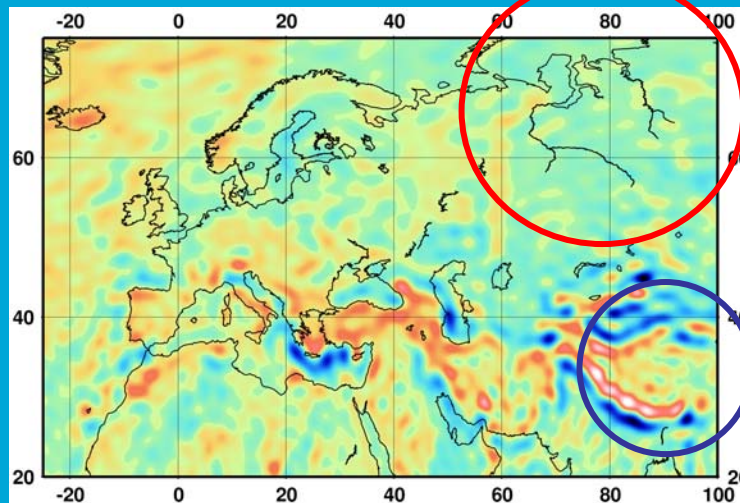
3) GRACE + surface until d/o 360 (EIGEN-GL04C)
