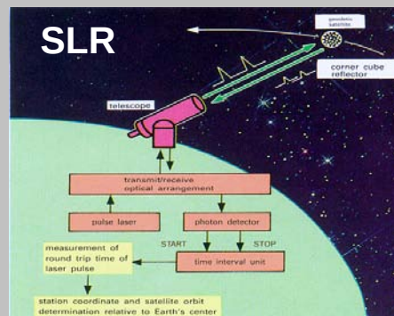
Satellite Laser Ranging
