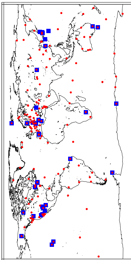
Current VLBI-GPS Collocations
