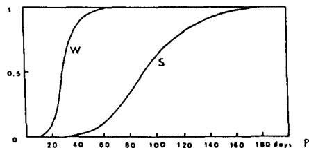
Figure 3 - Characteristics of the filters used for the BIH monthly operational solution (Circular D), 1984-1987.
